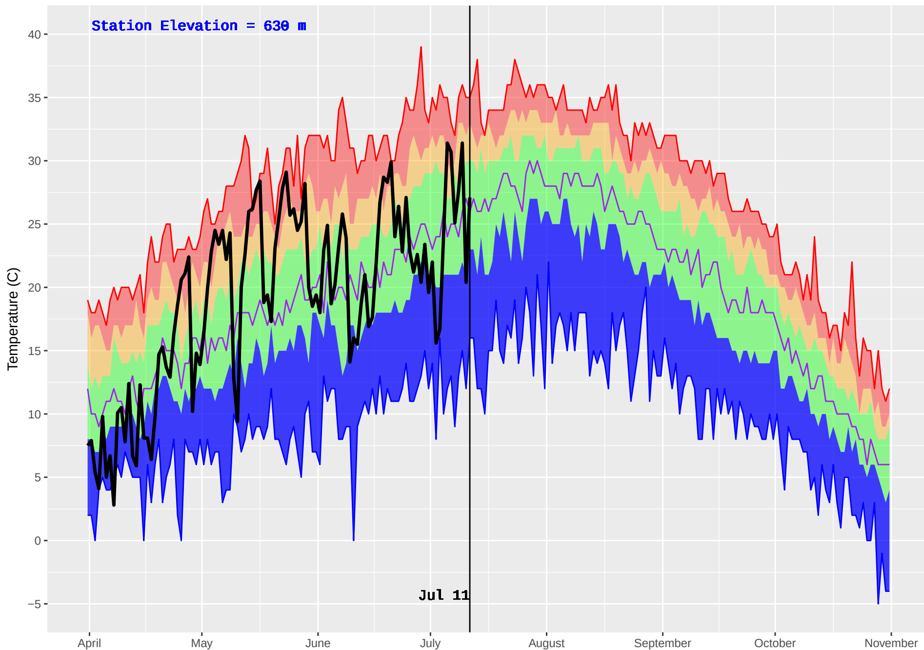
GRAND FORKS (392) : Historical (1981–2016) and Current (2018) Noon Temperature
