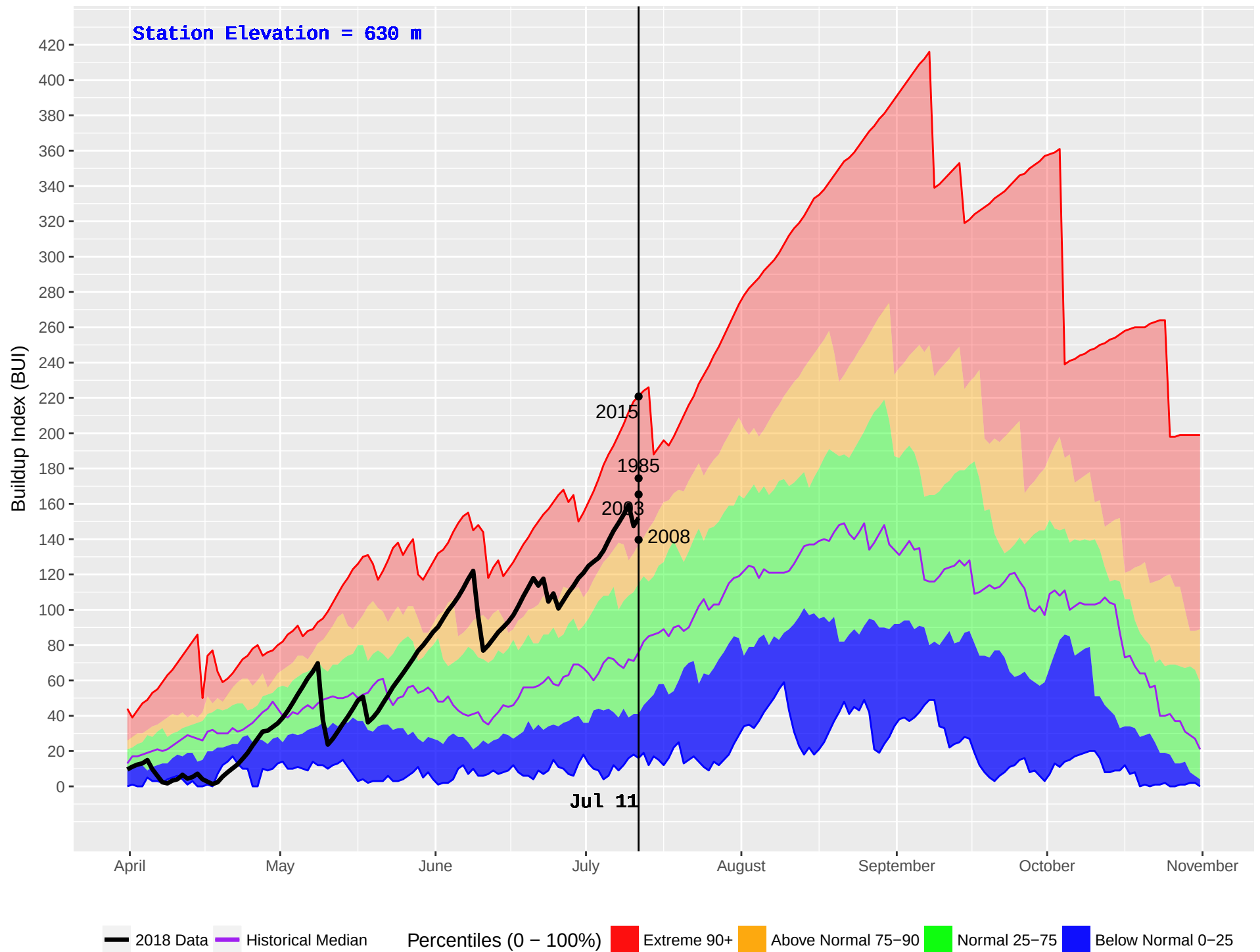
GRAND FORKS (392) : Historical (1981–2016) and Current (2018) Noon Buildup Index (BUI)
